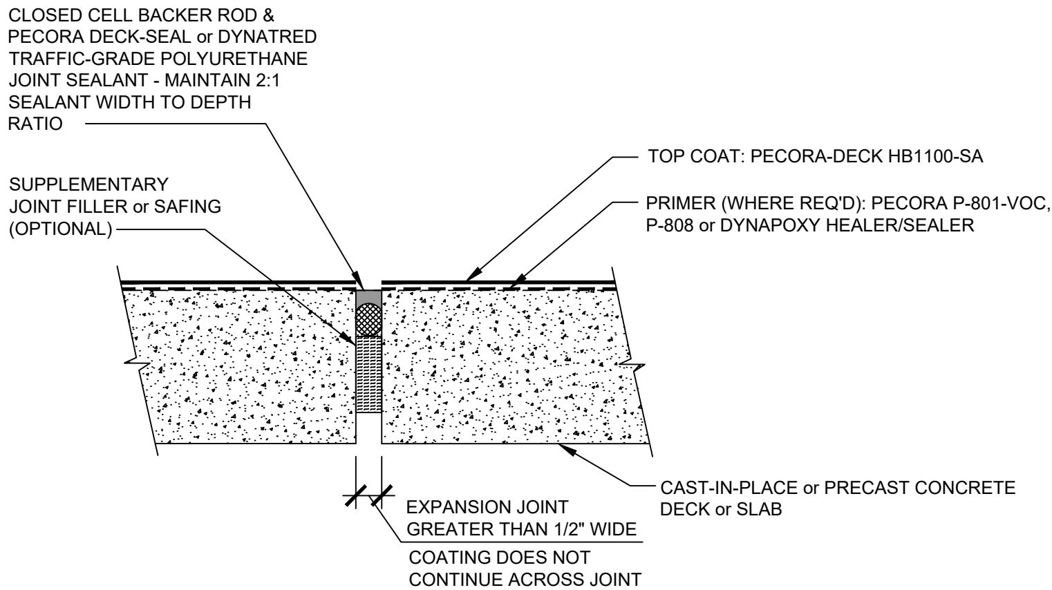
105: EXPANSION JOINTS > 1/2" WIDTH
